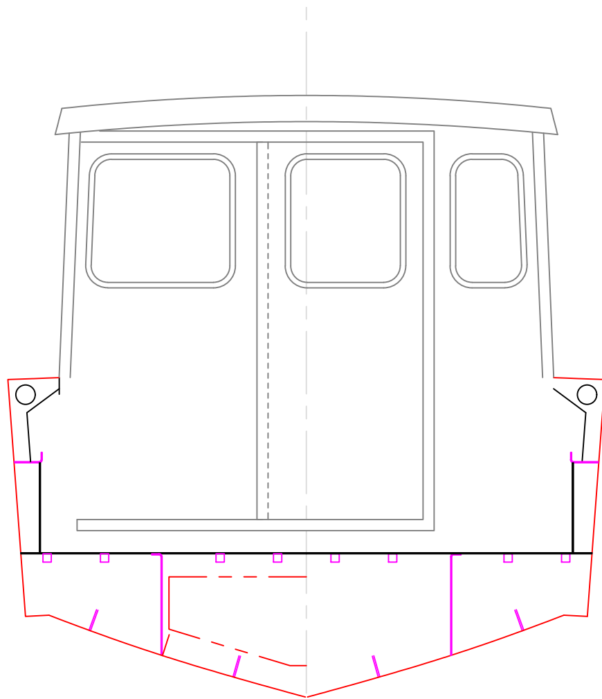
Frame 8 Lk'g Fwd
