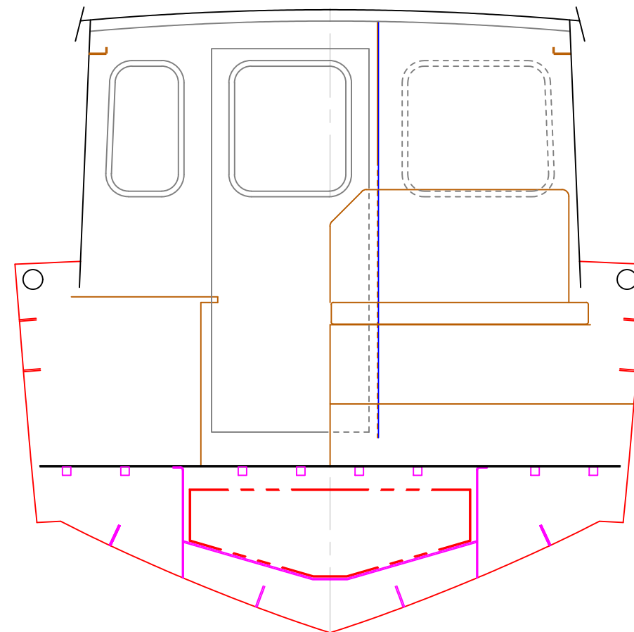
Frame 6 Lk'g Aft
