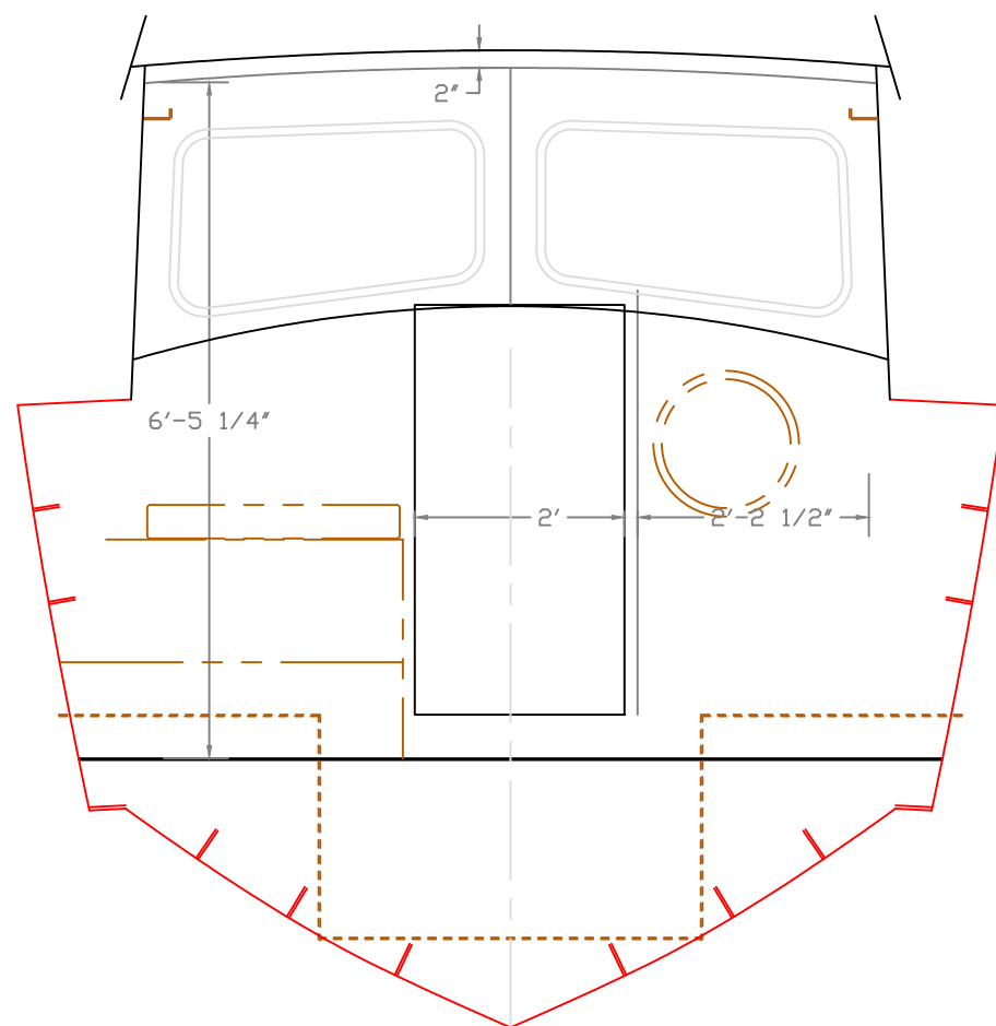
Frame 4 Lk'g Fwd
