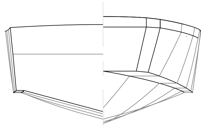
Representative Body Plan Not to Scale
